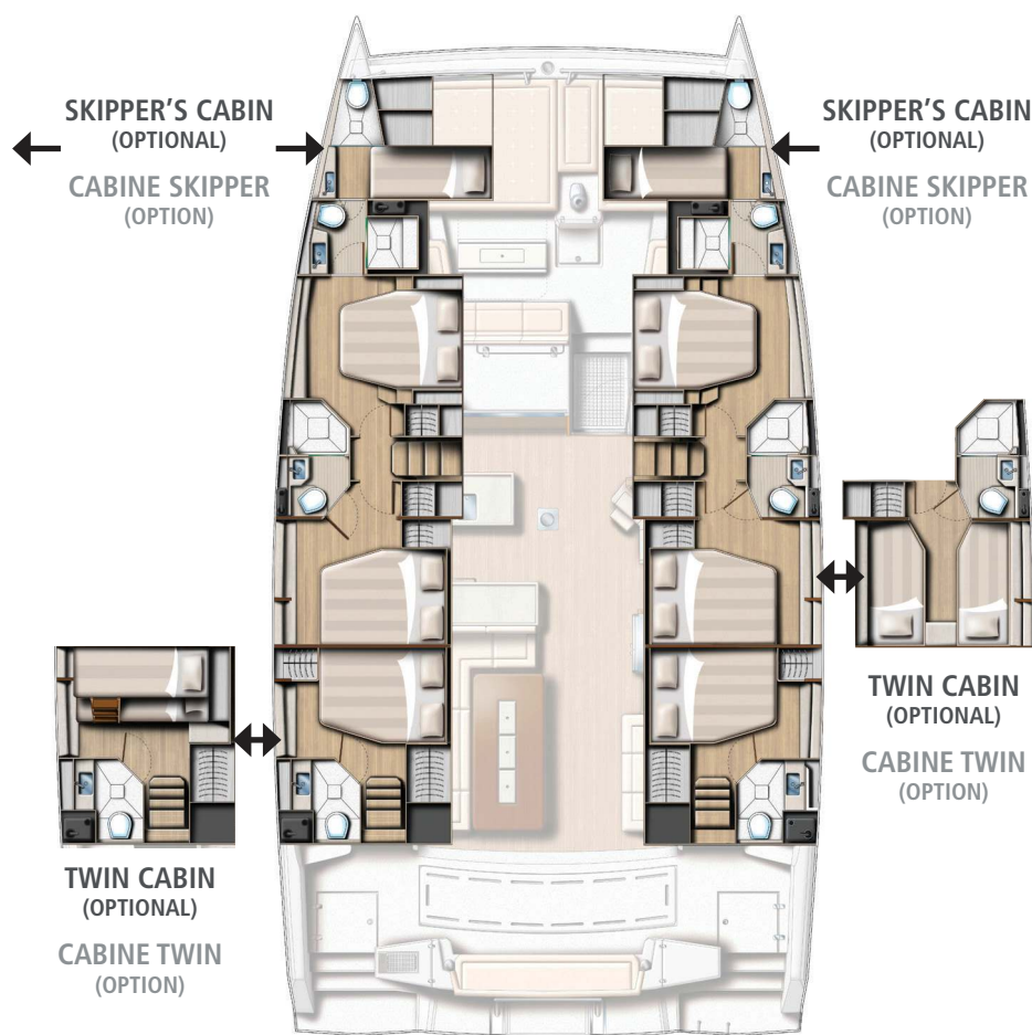
6 CABINS / 6 HEADS VERSION VERSION 6 CABINES / 6 SDB
